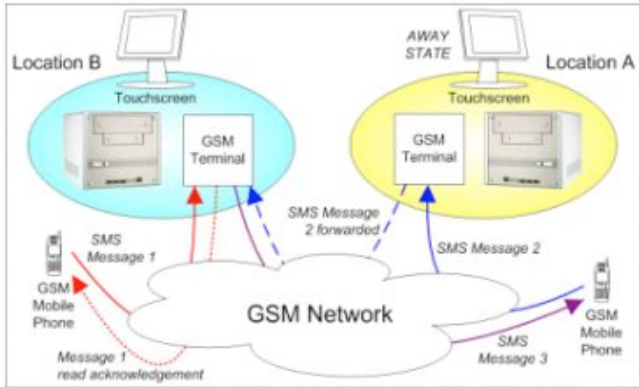
Figure 4. Architecture of the SPAM system
