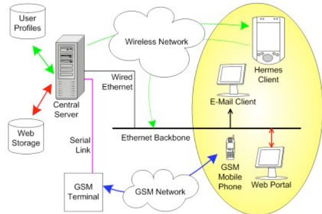
Figure 2. The System Architecture of Hermes [5]
